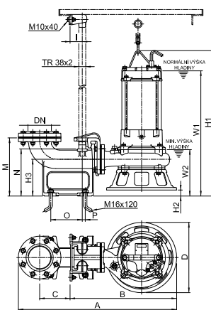
80SFP23.7 • 3" : ST80D
