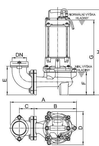
80SFU21.5 • 80SFU22.2
